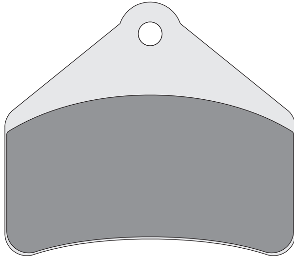
SDP851 78.1 × 69 × 11mm Brake Pad Compound Selection SDP Pro-SNX SDP851
