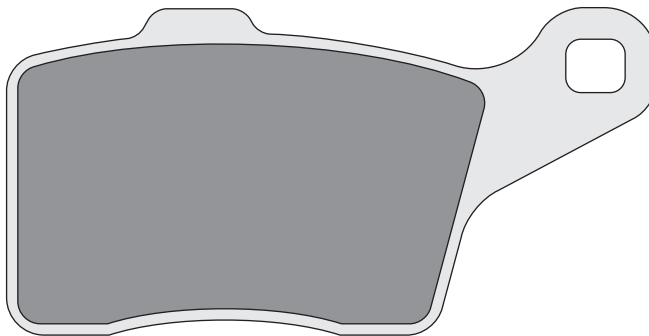
SDP852 86.4 × 43.4 × 99mm Brake Pad Compound Selection SDP Pro-SNX SDP852
