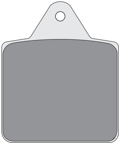
SDP844 50.2 x 60.8 x 12.3mm Brake Pad Compound Selection SDP Pro-SNX SDP844
