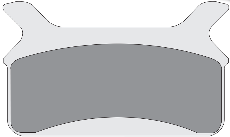
SDP845 102 x 62 x 9.7mm Brake Pad Compound Selection SDP Pro-SNX SDP845
