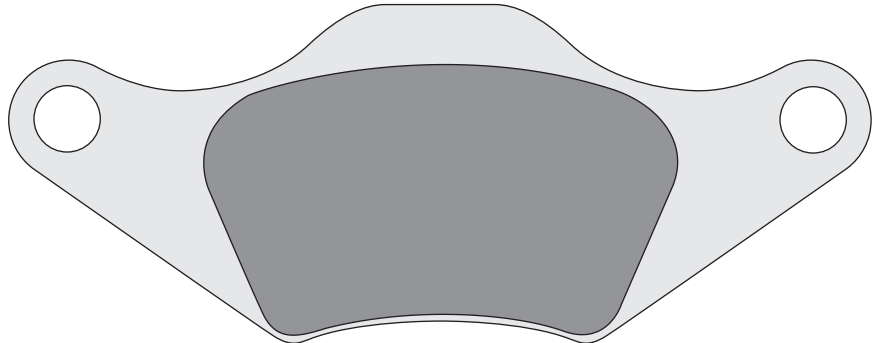
SDP849 115.6 x 45.2 x 10.5mm Brake Pad Compound Selection SDP Pro-SNX SDP849
